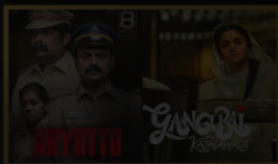
NAYATTU
